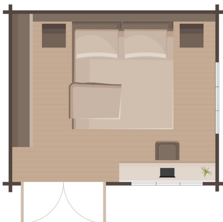
Meadow Solid Wood Cabin: 3.6 x 3m
